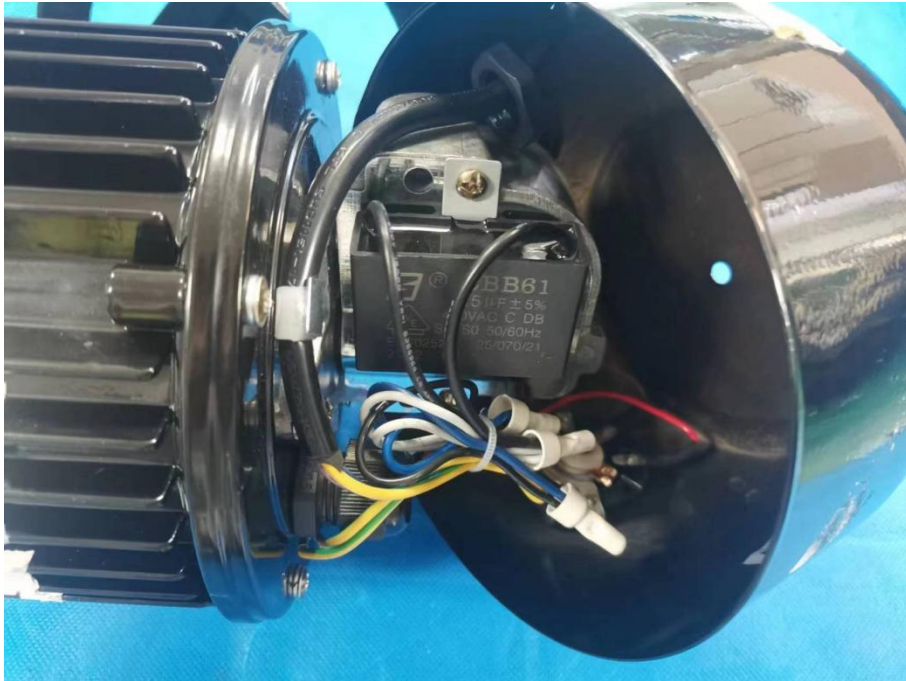
Figure 3:After the IP44 test ---End of Report---
